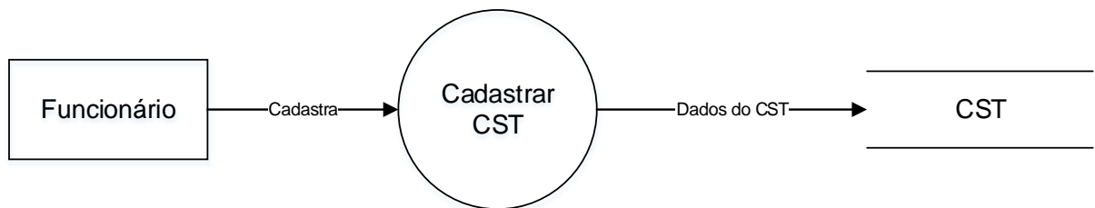
Figura 9 - DFD CST
