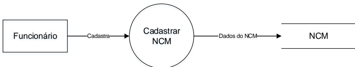
Figura 7 - DFD NCM
