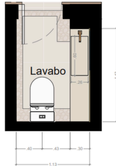
LAVABO LAYOUT
