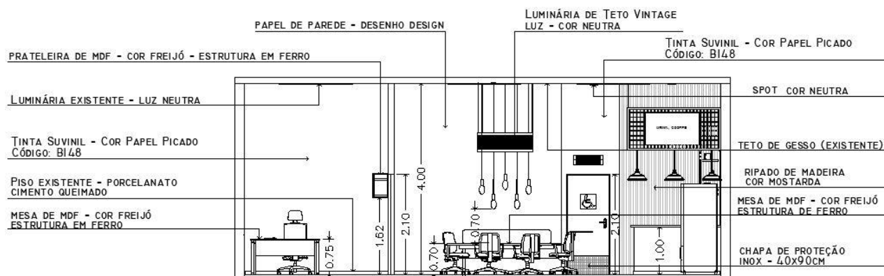
VISTA FRONTAL - COWORKING TWO HOUSE SEM ESCALA
