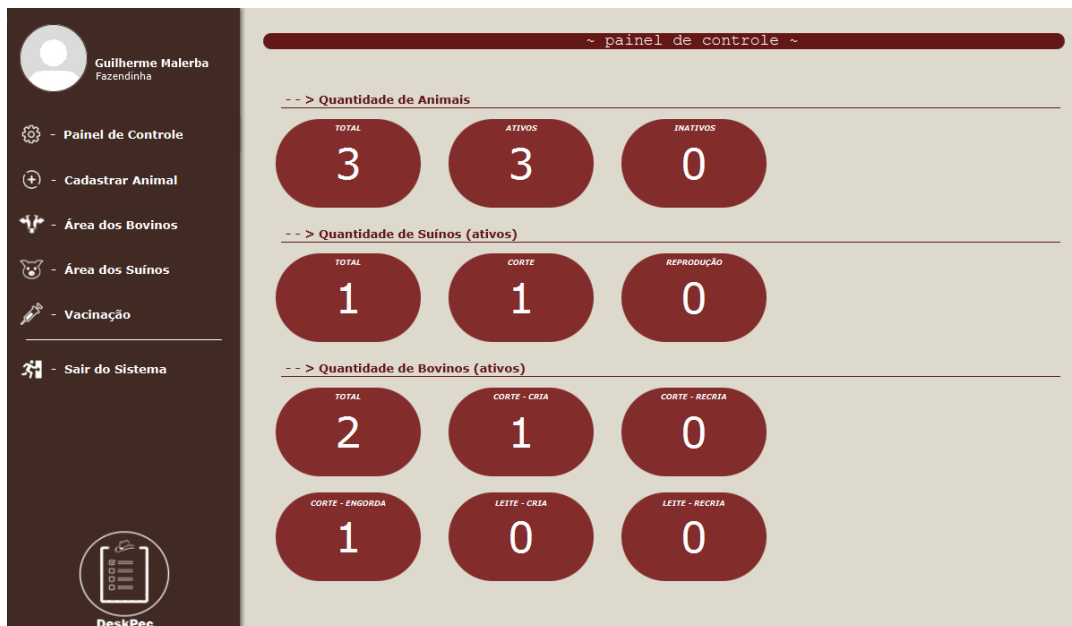
Figura 13 – Tela principal
